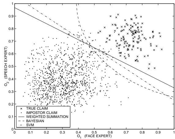
Figure 6: Decision boundaries used by fixed post-classifier fusion approaches and the distribution of opinion vectors for true and impostor claims (clean speech).
