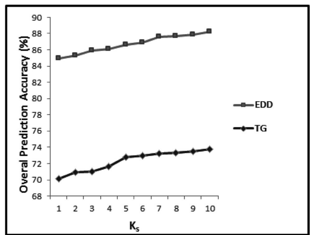
(a) The impact of increasing K_s from 1 to 10 while K_p = 1 for EDD and TG data sets.
