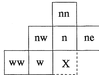
Figure 2. The Prediction context of pixel X
